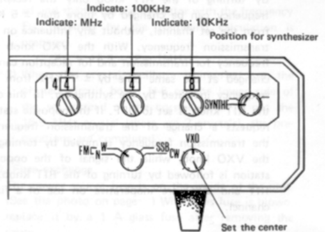
HOW TO READ THE FREQUENCY (Fig. 144.480MHz)
